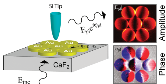
Figure 2. Principle of near-field imaging of a plasmonic structure (here a mid-infrared-resonant oligomer structure composed of seven gold disks) by s -SNOM (left). The light scattered by the tip is detected by an amplitude- and phase-resolving interferometer, yielding near-field amplitude and phase images (right). While the amplitude image shows the dipolar plasmon modes on each disk, only the phase image reveals the relative phase shift between them. The central disk oscillates out of phase with the outer disks, revealing the subradiant (“dark”) character of the mode.
