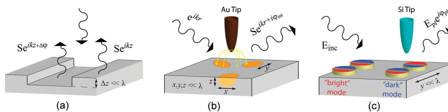
Figure 1. Phase plays three important roles in nanooptics. (a) Far-field determination of nanoscale differences in surface height, or, alternatively, sample thickness may be accomplished through phase-sensitive measurements. The phase varies over a 2\pi range. (b) Near-field investigation of material properties. Local interactions between the metal tip and the sample, which provide strong field concentration, change the phase of the scattered field allowing local identification of materials at nanoscale. (c) Near-field mapping of surface modes. Mapping phase of the local field distribution enables direct investigation of the modes in plasmonic nanostructures. The role of the tip is to out-couple the local field to the detector, therefore dielectric tips, which minimize the field disturbance due to the tip presence, are preferred. 28
